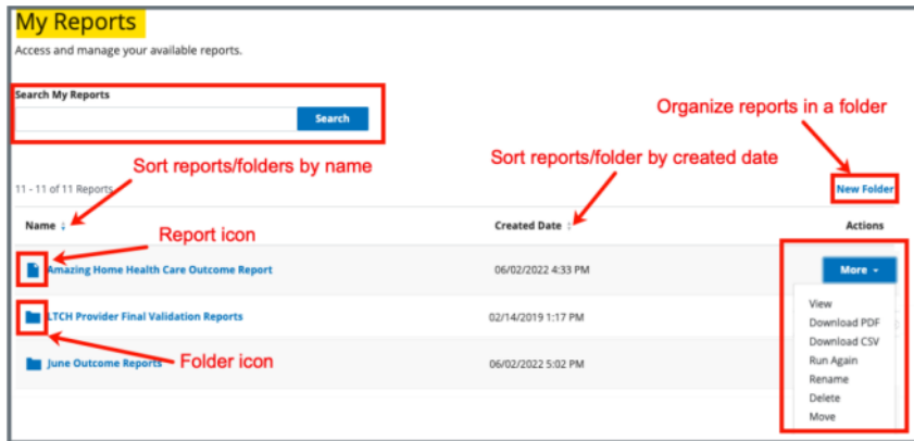
Figure 19: My Reports
